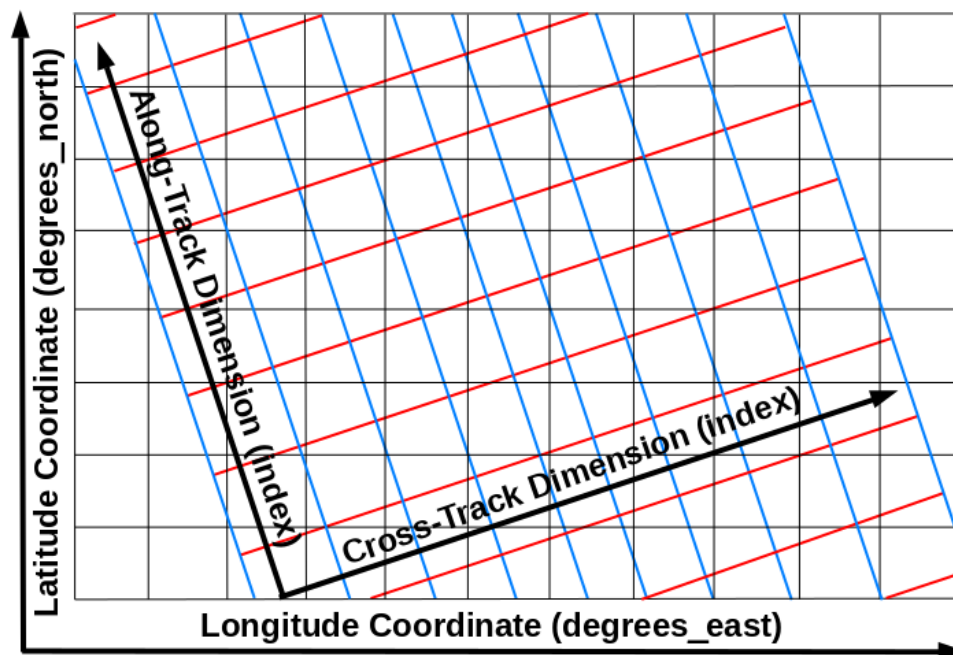
Figure 2 The horizontal dimensions (along_track and cross_track) and coordinates (latitude and longitude) for a sun-synchronous swath product. In some products the horizontal dimensions and coordinates can be one and the same (i.e., latitude and longitude).
