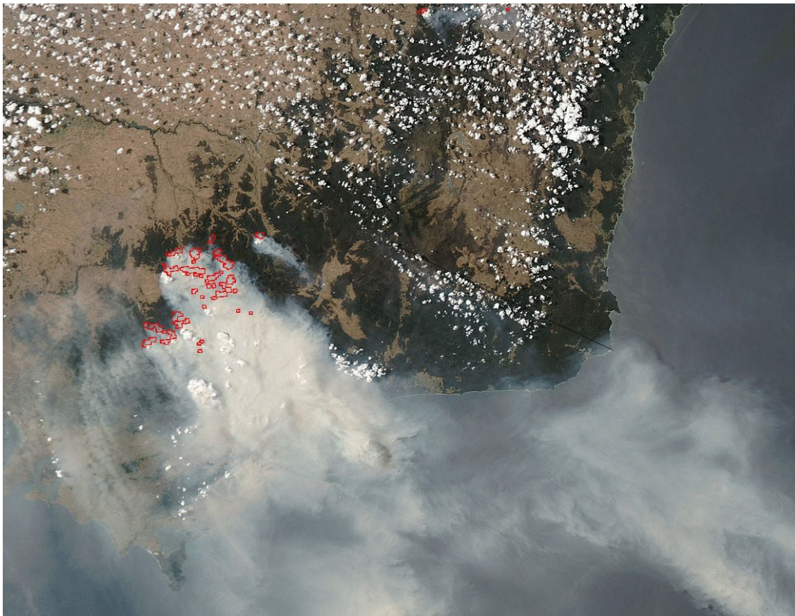
Figure 7: LANCE true color imagery of fires and smoke in southeast Australia (10 December 2006, 03:45 UTC).
