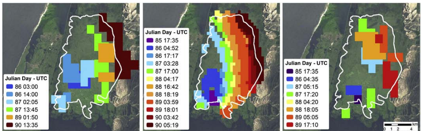
Fig. 9. Daily fire spread mapped by 1 km Terra/MODIS (left), 375 m VIIRS (center), and 1 km Aqua/MODIS (right) data for a wildfire at the Taim Ecological Reserve in southern Brazil ( -32.7^{\circ} lat, -52.55^{\circ} lon). The data cover the period beginning on 26 March 2013 (Julian day 85) and ending at the approximate time of the Landsat-7 data acquired at 13:15UTC on 31 March 2013. The white vector outline represents the burned area mapped using the 30 m Landsat-7 data.
